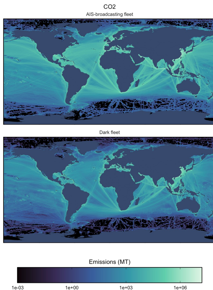
Figure 7. Map of 2025 CO 2 emissions, aggregated across all vessel classes, at 1x1 degree spatial resolution, disaggregated by the dark fleet and AIS-broadcasting fleet.
