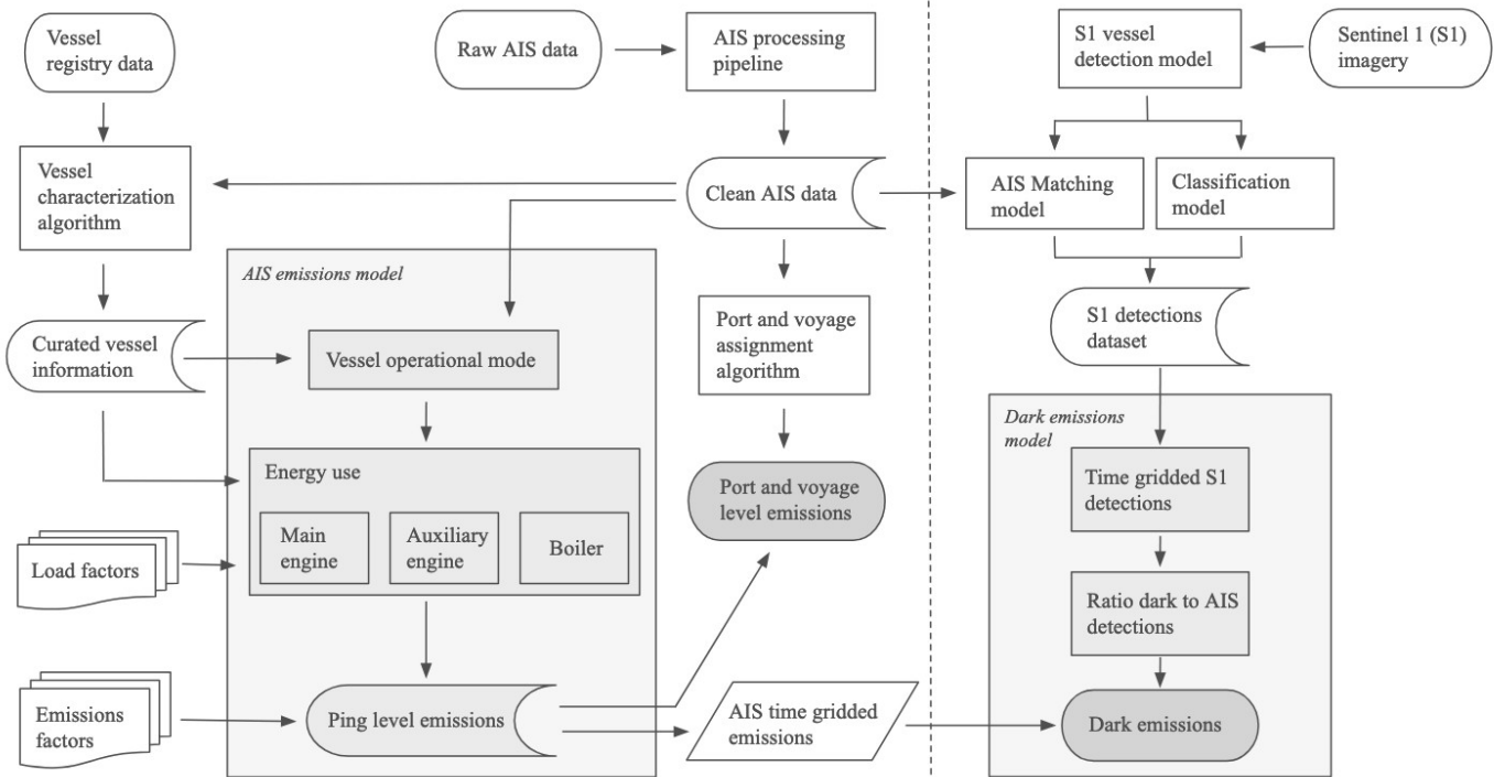
Figure 1. GFW framework for estimating emissions using the AIS-based emissions model and the non-broadcasting (dark vessel) emissions model.
