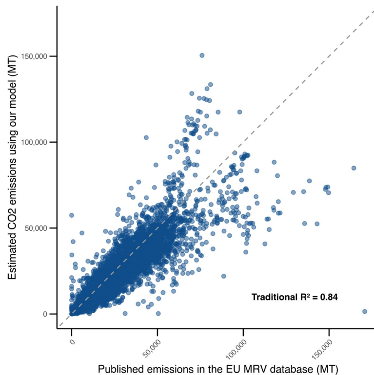
Figure 4. Comparison of annual vessel-level CO 2 emissions estimated using our AIS-based model with published emissions from the EU MRV database (EMSA, 2025). The sample includes 27,657
