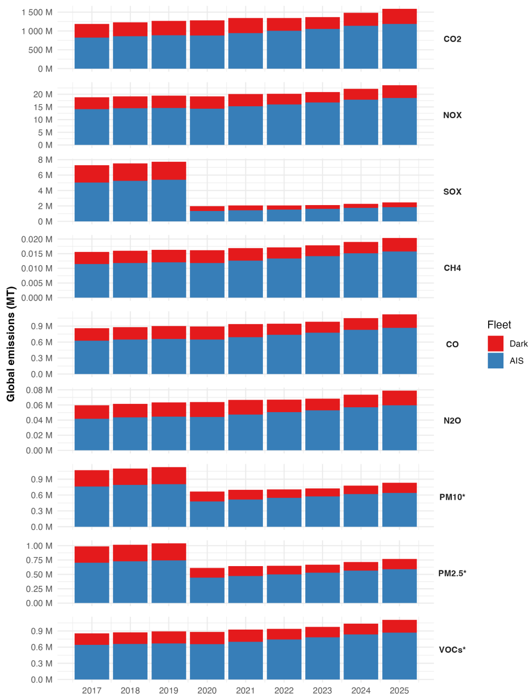
Figure 6. Summary of total global annual emissions over time, by pollutant and fleet. All emissions units are in metric tonnes, disaggregated by the AIS-broadcasting fleet and the dark fleet as detected by S1.
