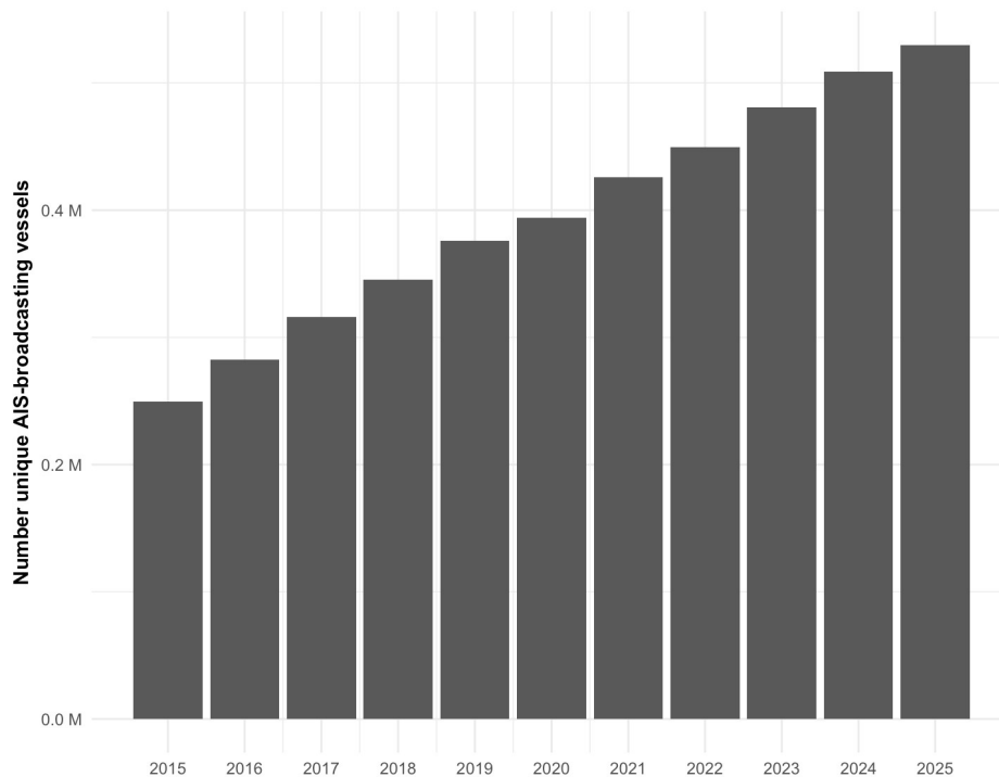
Figure 5. Total number of AIS-broadcasting vessels, by year, for which we estimate emissions.
